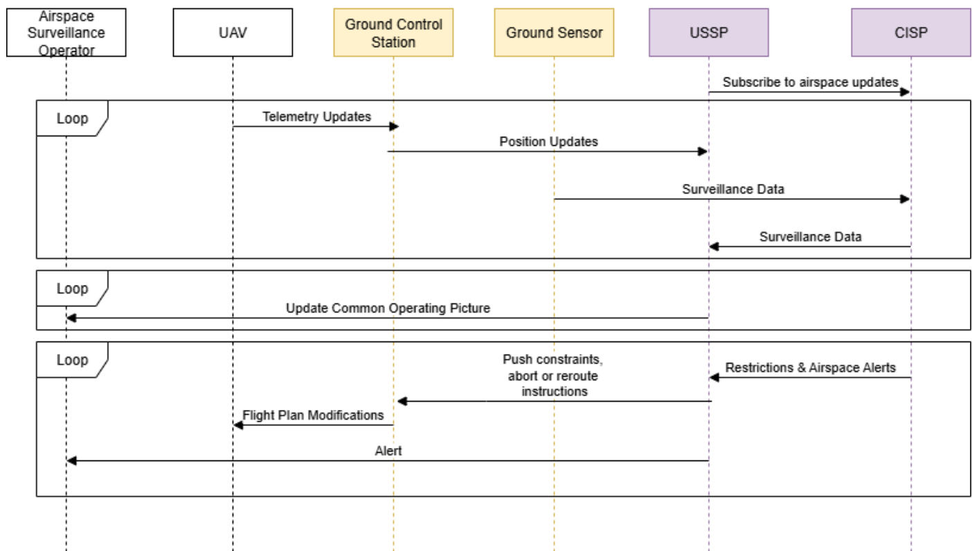
Figure 8.3: Unmanned Airspace Surveillance Information Flow
