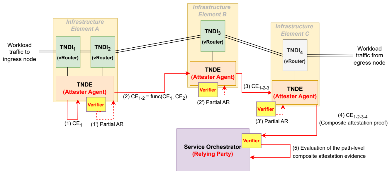
Figure 3.5: Composite attestation in a cascading multi-prover/multi-verifier scenario. The TNDE's Attestation Source of each path element contribute to the creation of a composite attestation proof that captures the state of an established network path.
