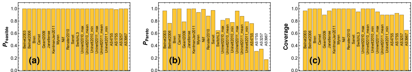
Figure 5.7: Statistical performance of bSB across real network topologies. Panels (a)– (c) report the feasibility probability, Pareto hit probability, and Pareto coverage averaged over ten source–destination instances for each topology.
