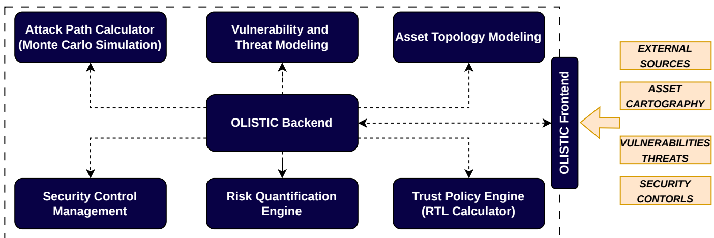
Figure 4.1: CASTOR Risk Assessment Engine
